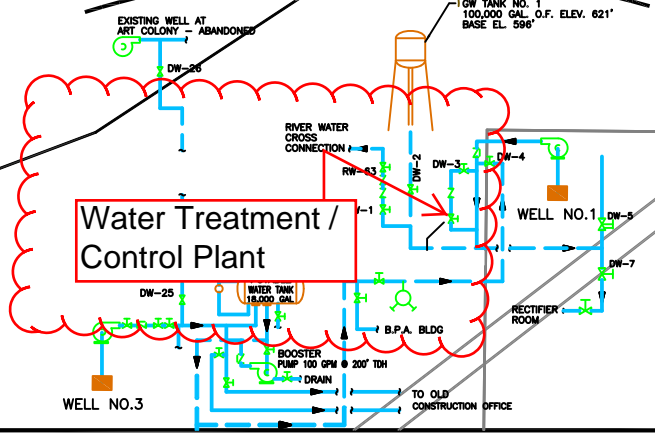
FIGURE 5-1 SW SYSTEM IMPROVEMENTS
