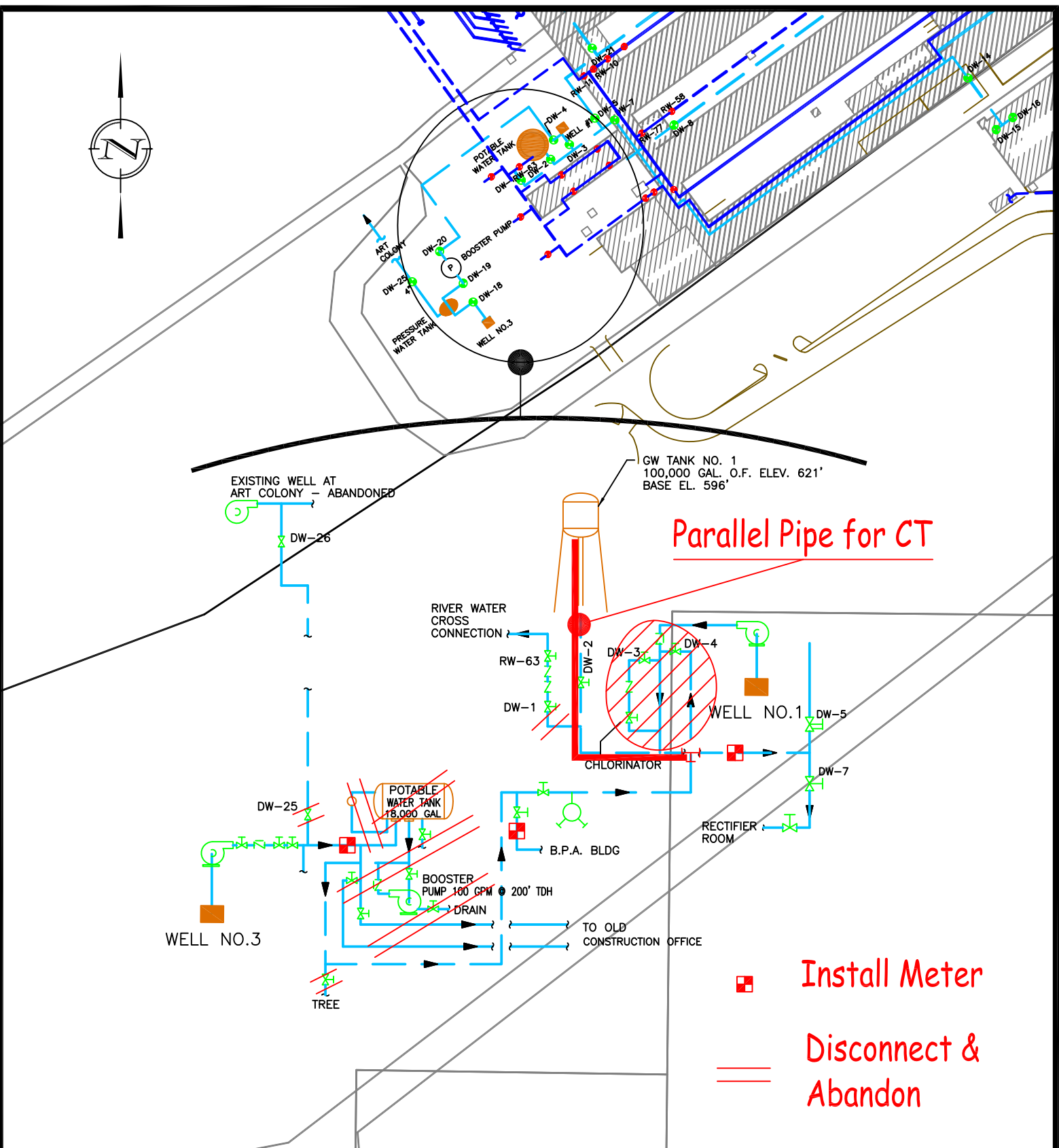
FIGURE 5-2 GW SYSTEM CIP
